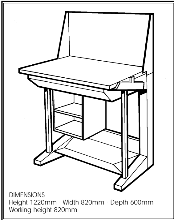
Combined Welding & Cutting Surface
